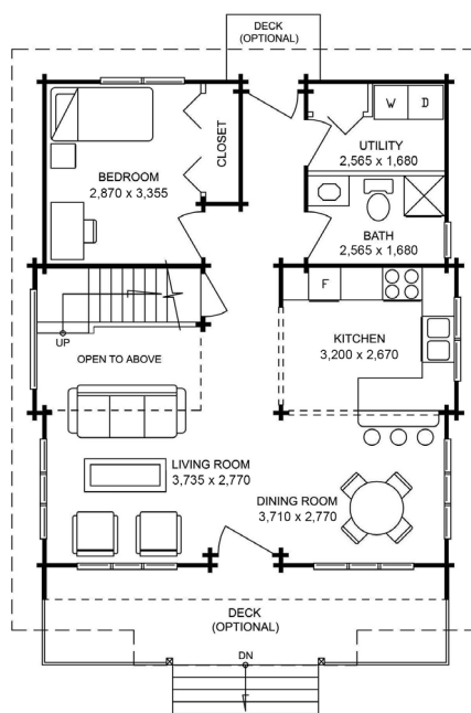
MAIN FLOOR 70.30 m 2
