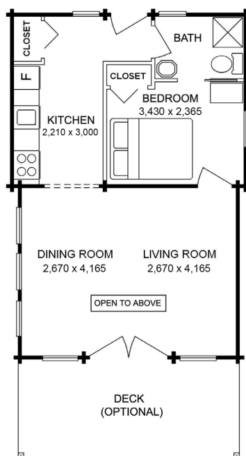
MAIN FLOOR 49.29 m 2
